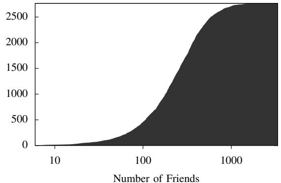
Figure 6. Distribution of users' number of friends.
