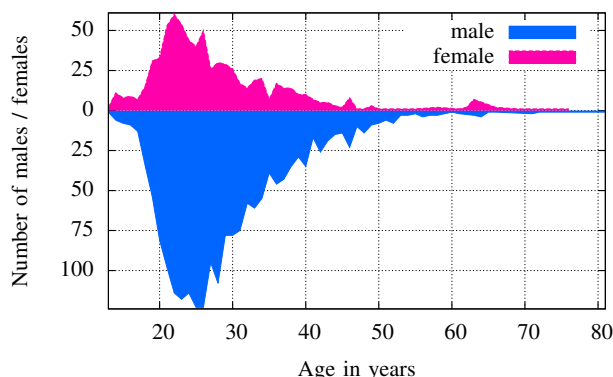
Figure 5. Densities of ages of male and female participants.
