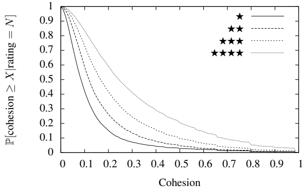
Figure 8. Normalized reversed cumulative distribution of cohesion for groups rated 1,2,3 or 4 stars ( \mathbb{P}[\text{cohesion} \geq X | \text{rating} = N] ).
