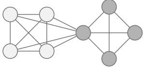
Figure 1. Two sets of nodes of identical size, featuring the same number of links both inside the set and towards the rest of the network. Despite those structural similarities, the darker set appears to be a better community than the lighter one.
